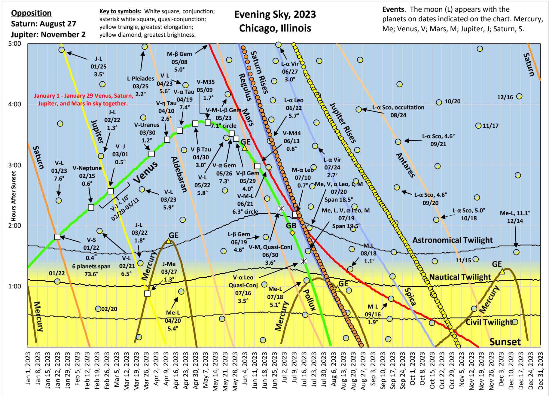
All moon dots, and the curves for planets and stars, indicate setting times in relation to sunset, except for the two planet curves labeled to indicate times of rising, also in relation to sunset.
